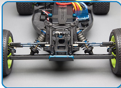
Updated shock towers optimized for the 12mm "Big Bore" shocks
