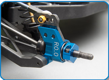
Factory Team 7075-T6 blue aluminum 0° rear hubs with oversized outer bearing
