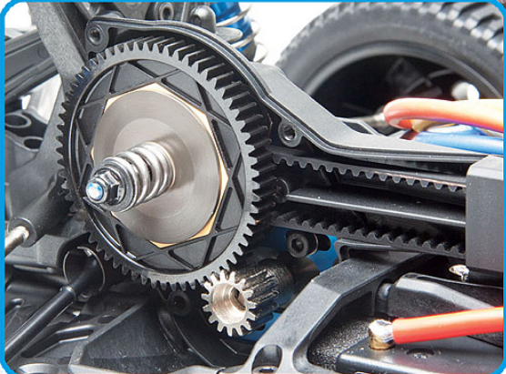
Decoupled center slipper clutch allows for front and rear wheel drive to slip independently, resulting in more traction and stability on bumpy track conditions
