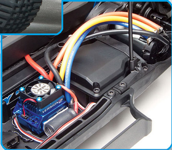
Sealed water-resistant receiver box and removable ESC tray for easier maintenance. Uses most 540 and 550 brushless motors.
