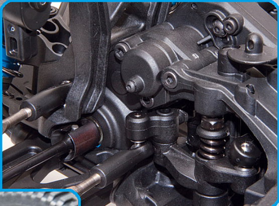
Unique dual gearbox drive train coupled together with a 5mm heavy duty belt system with external tension adjustment. 32-pitch front and rear gearboxes with sealed fluid-filled differentials.
