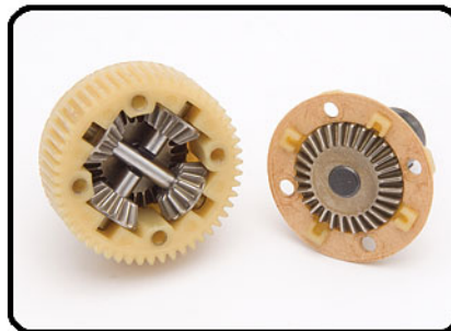
2.6:1 gear ratio gearbox with sealed gear differential
