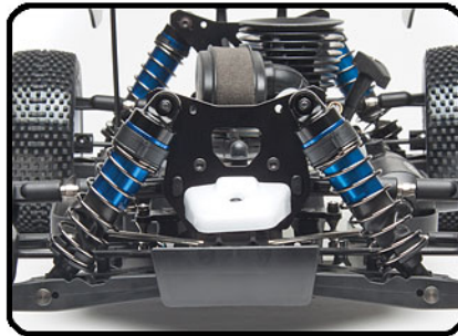
Updated RC8.2 racing suspension geometry
