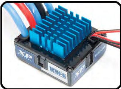
New high-power water-resistant XP SC700 with Deans® Ultra Plug® battery connector
