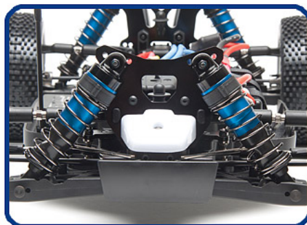
Updated RC8.2 racing suspension geometry
