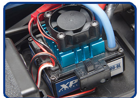
Waterproof XP SC1300-BL brushless ESC
