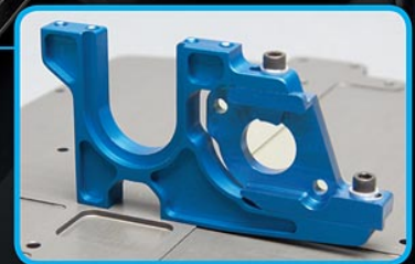
Machined 7075-T6 blue aluminum floating motor mount
