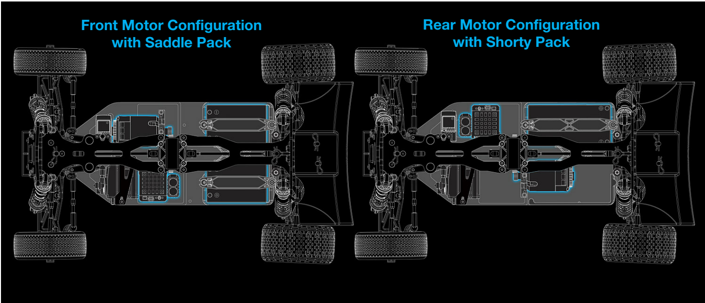
Weight bias can be significantly altered by using either the front motor configuration with a saddle pack (left) or the rear motor configuration with a shorty pack.
