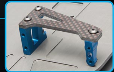
New floating servo mount improves symmetrical chassis flex
