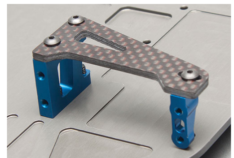
New floating servo mount
