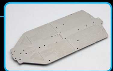
Hard anodized aluminum chassis allows for front or rear motor configurations
