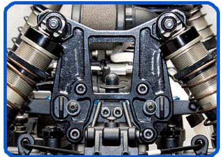
Factory Team 7075 aluminum low-center-of-gravity shock towers with optimized geometry
