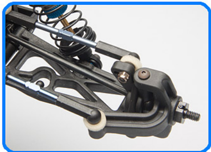
Complete set of Factory Team blue titanium turnbuckles
