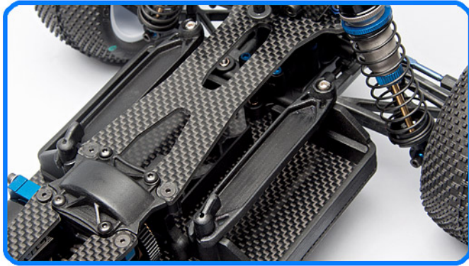
Composite battery trays with integrated spacers and quick-change battery straps
