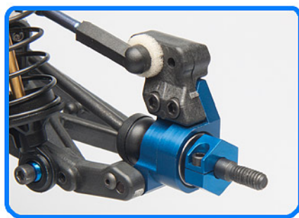
Factory Team 0° aluminum rear hubs with 12mm clamping hexes
