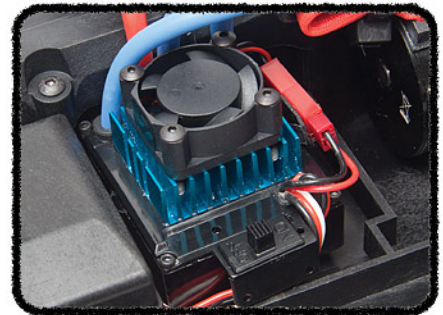
XP water-resistant LiPo compatible electronic speed controller
