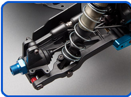
Newly designed suspension arms feature centerline shock mounts and optimized anti-roll bar position
