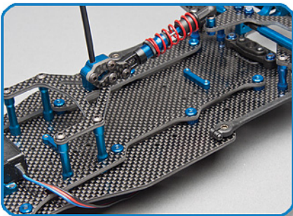
Ultra-rigid 2.5mm thick carbon fiber chassis with integrated chassis stiffening rails
