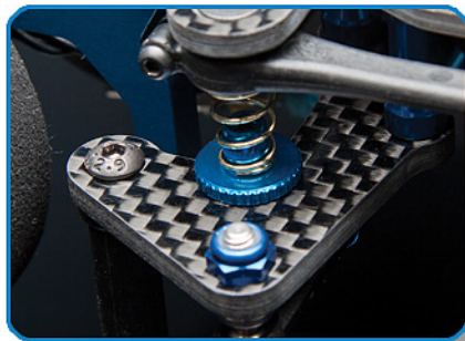
Aluminum side spring retainers
