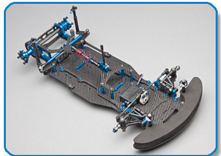
Engineering excellence to take on the 1:10 scale World GT on-road racing class
