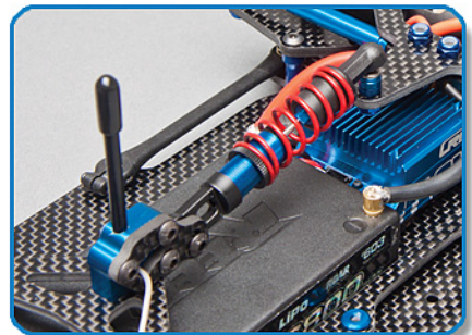
Innovative through-shaft center shock
