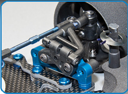
Dynamic Strut front suspension features symmetrical components
