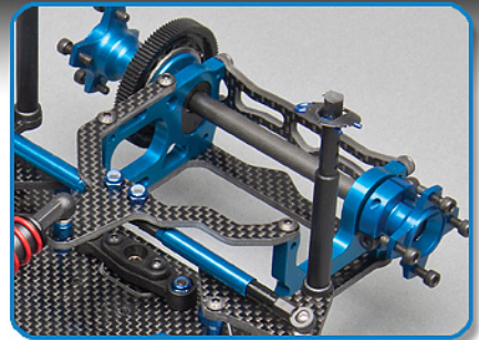
3-point upper pod plate with graphite motor mount cross-brace
