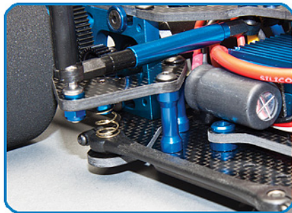
Pivot-ball rear pod design
