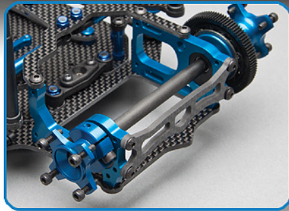
Updated motor mount and left rear bulkhead
