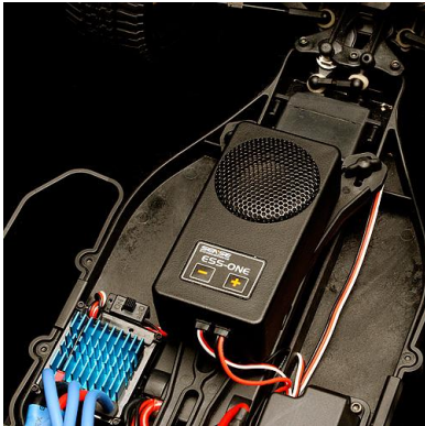
#29260 ESS-One Engine Sound System installed in the SC10
