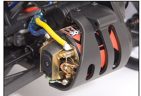
17-turn Reedy motor.
