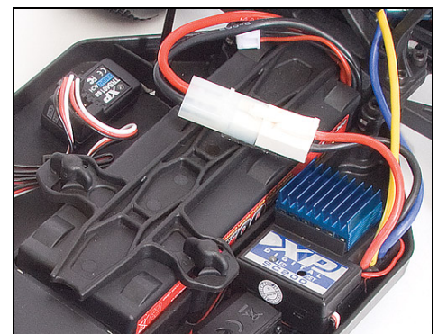
Battery strap with twist-lock thumb knobs.
