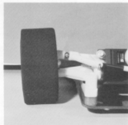
positive camber
