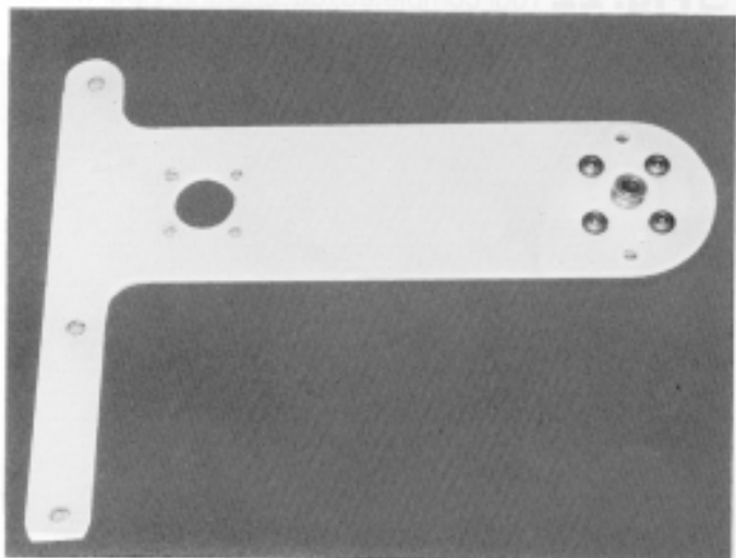
underside of T-bar
