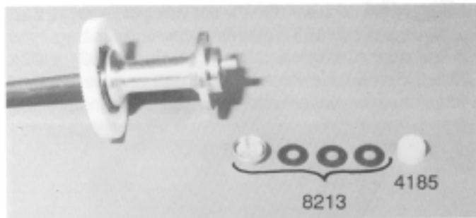
#8213 diff thrust cone #8213 belleville washers #4185 8-32 nylon locknut
